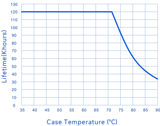
Lifetime Vs. Case Temperature
