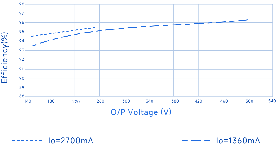
Efficiency Vs. O/P Voltage (Vin=347Vac)
