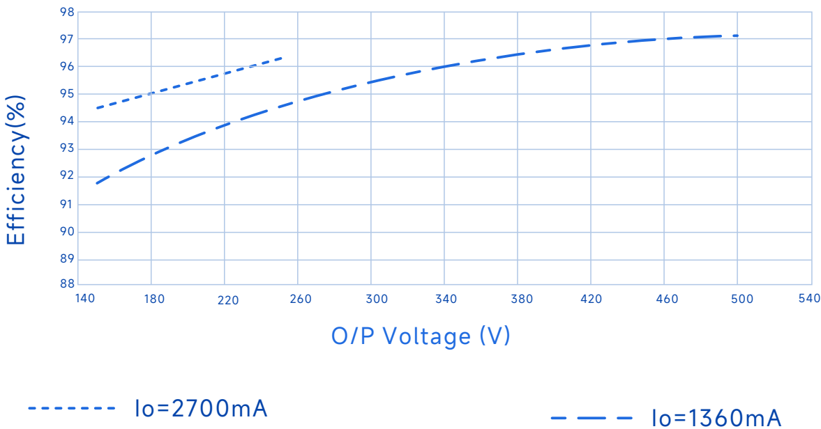
Efficiency Vs. O/P Voltage (Vin=480Vac)
