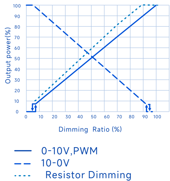
O/P Power Vs. Dimming
