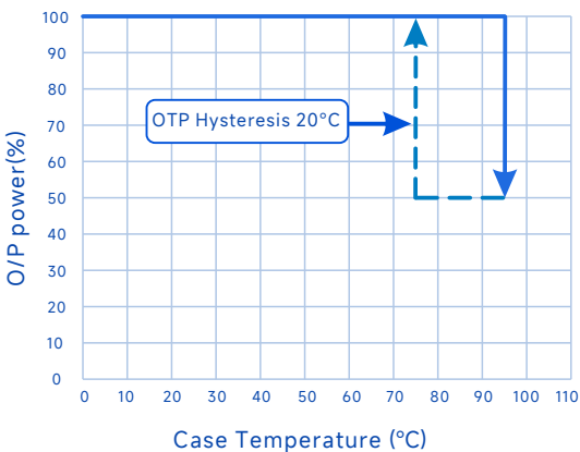
O/P Power Vs. Case Temperature
